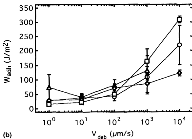
FIGURE 8 Adhesion energy, W_{adh} , as a function of debonding rate at different temperatures ( \circ — 50^\circ\text{C} , \square — 20^\circ\text{C} , \diamond — 0^\circ\text{C} , \triangle — -20^\circ\text{C} ) for (a) PEHA and (b) PEHA-AA as a function of debonding rate.
