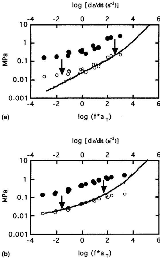
FIGURE 23 Comparison between the shear storage modulus, G' ( a_T g ) (—) and maximum stress, \sigma_{\max}(d\varepsilon/dt) for (a) PEHA and (b) PEHA-AA. The correspondence between a_T f and d\varepsilon/dt was set based on reasonable assumptions explained in the text. The filled symbols represent the actual value of \sigma_{\max} while the unfilled symbols are the best fit to the shear modulus data ( \sigma_{\max} = 10 G' for both PEHA and PEHA-AA).
