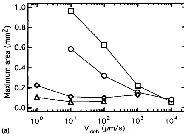
FIGURE 17 Maximum average area of a cavity, projected in the plane of the film, as a function of debonding rate at different temperatures (—○— 50^{\circ}\text{C} , —□— 20^{\circ}\text{C} , —◇— 0^{\circ}\text{C} , —△— -20^{\circ}\text{C} ) for (a) PEHA and (b) PEHA-AA.
