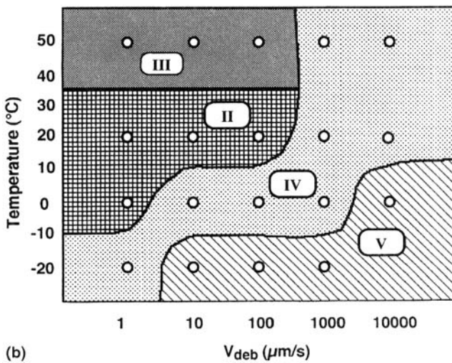
FIGURE 13 Map of the different types of curves observed as a function of temperature and debonding rates for (a) PEHA and (b) PEHA-AA. The circles represent the actual rates and temperatures of our tests.
