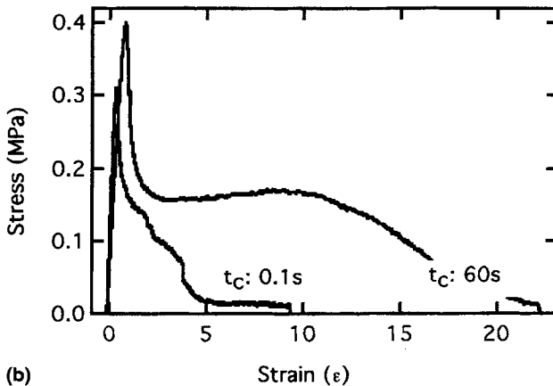
FIGURE 18 Stress–strain curves obtained at: (a) 0.1 s (—○—), 1s (—■—) and 60s (—) contact time at 50°C and (b) 0.1 s and 60s contact time at –10°C for the PEHA-AA polymer at a debonding rate of 10 \mu\text{m/s} .
